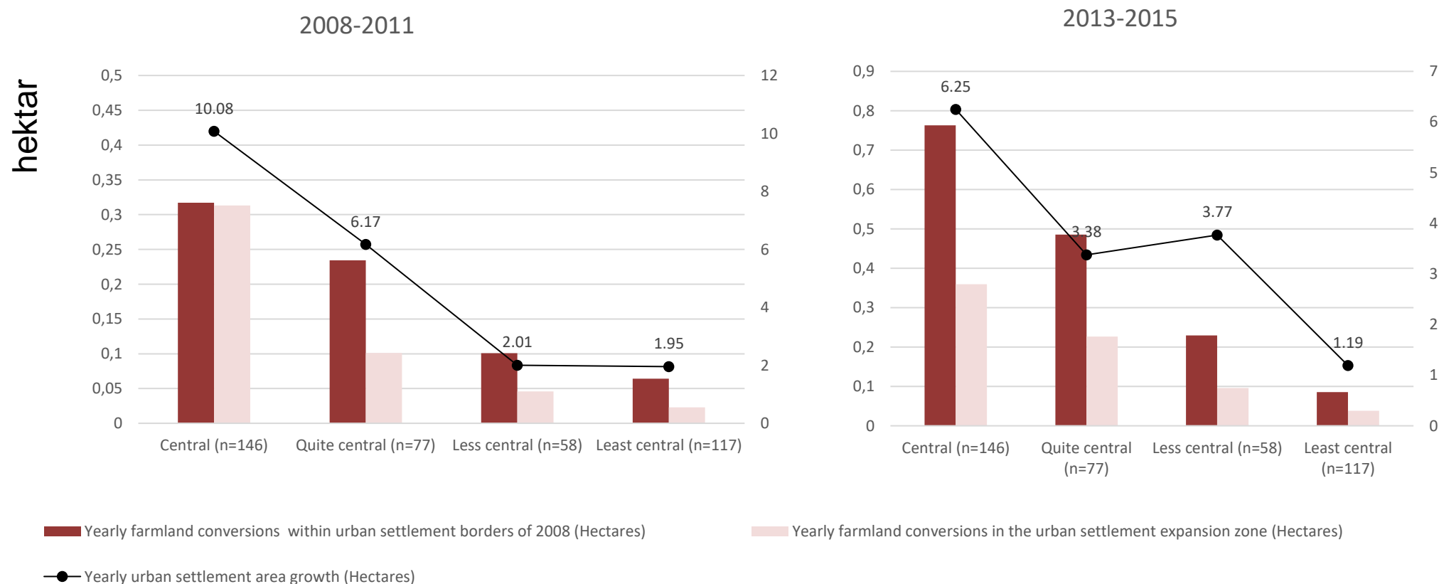
Fig: Yearly urban settlement land expansion and the corresponding conversion of farmland in the periods 2008–2011 and 2013–2015 in municipalities with different centralities (hectares per municipality). N = 398 municipalities.
