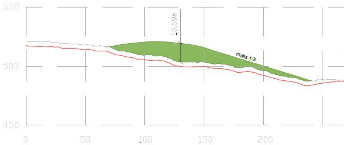
Snitt A-A' massedeponi BAA4, 1:1000
